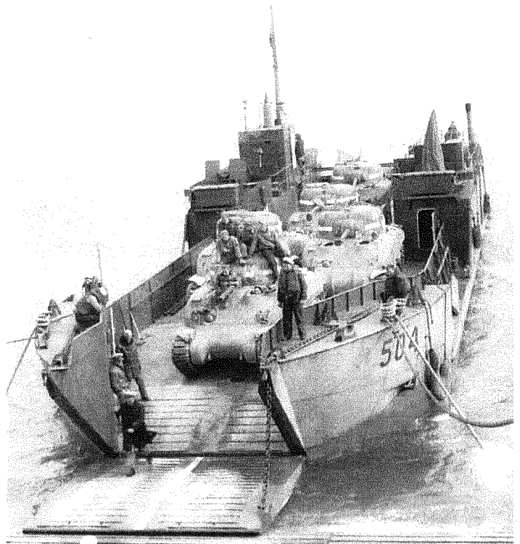
LCT(6) 504 prepares to unload tanks into the bay of an LCD in the European Theater. NARA
